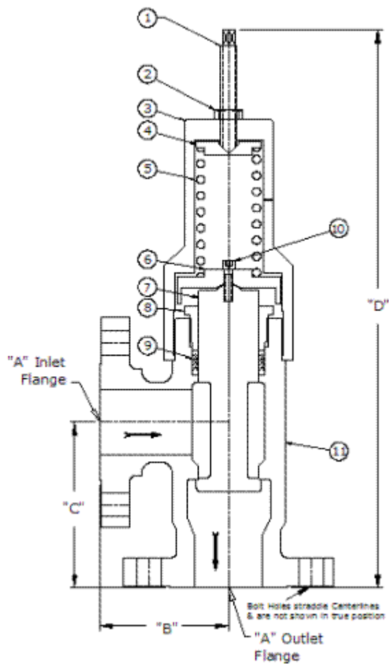
Model PRH-04-600#Fig
