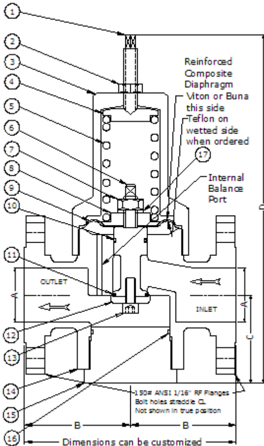
PRS09i-Flg Soft Seated
